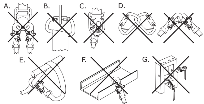
Figure 4 - Making Connections
