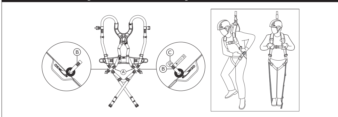
Figure 12 - Activation des sangles anti-traumatisme
