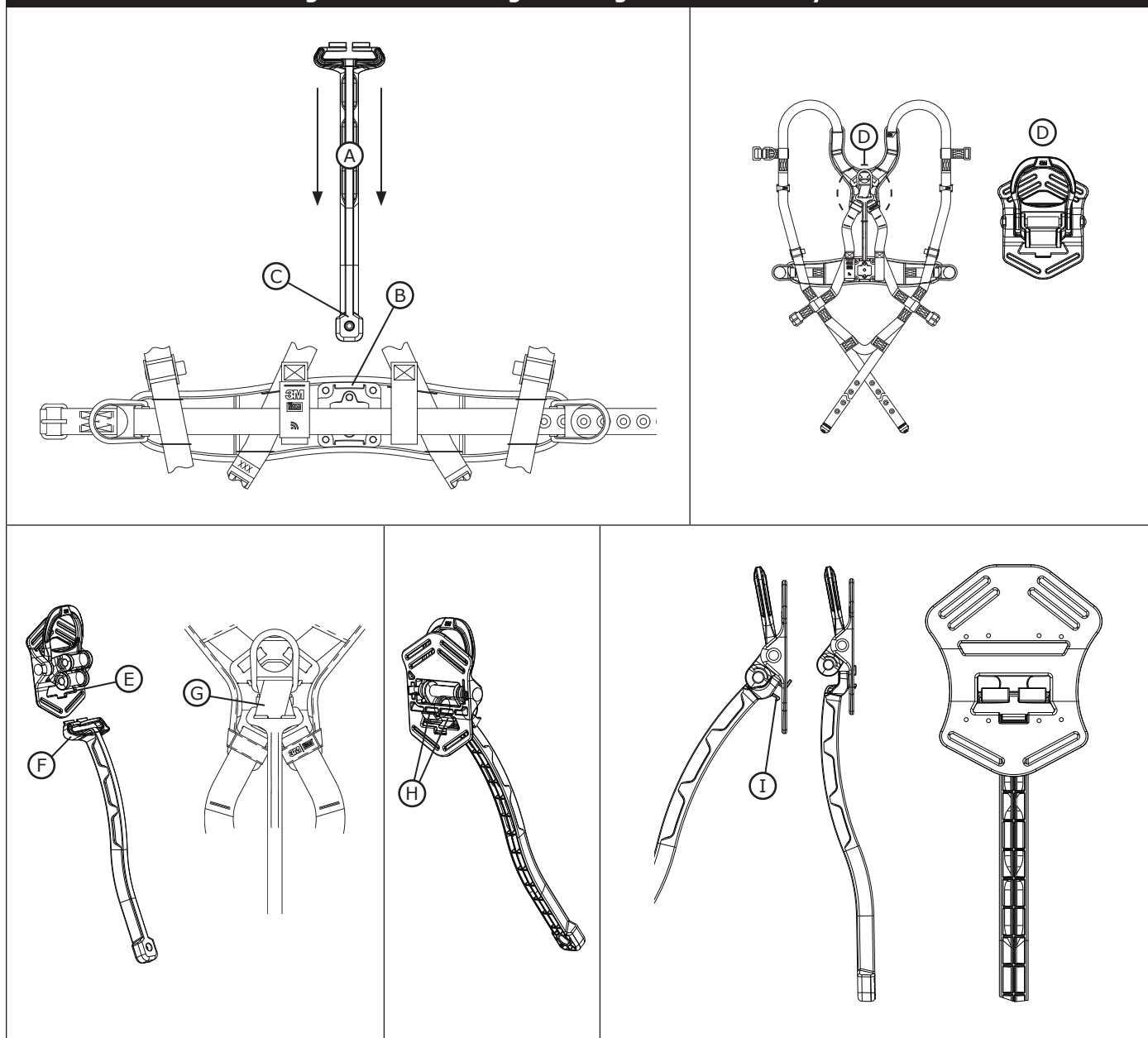
Figure 11 - Attaching the Weight Distribution System
