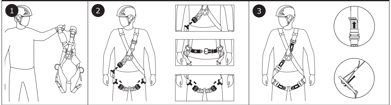
Figure 6B - Donning the Crossover-Style Harness
