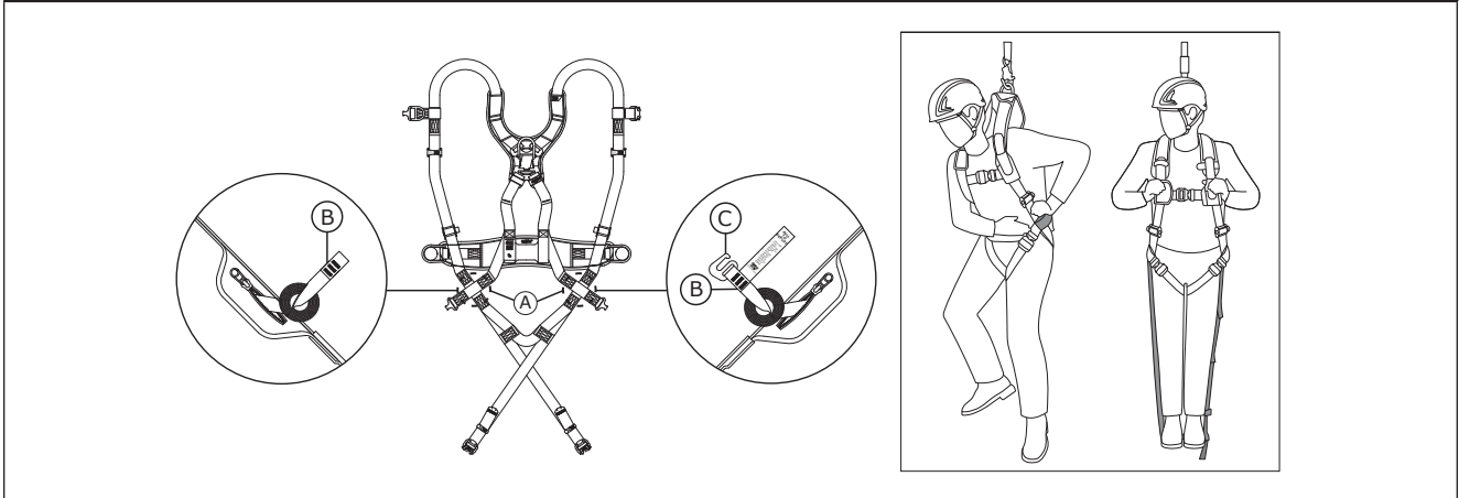
Figure 11 - Activation des sangles anti-traumatisme
